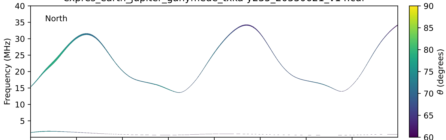
expres_earth_jupiter_ganymede_txka-y235_20330621_v14.cdf
