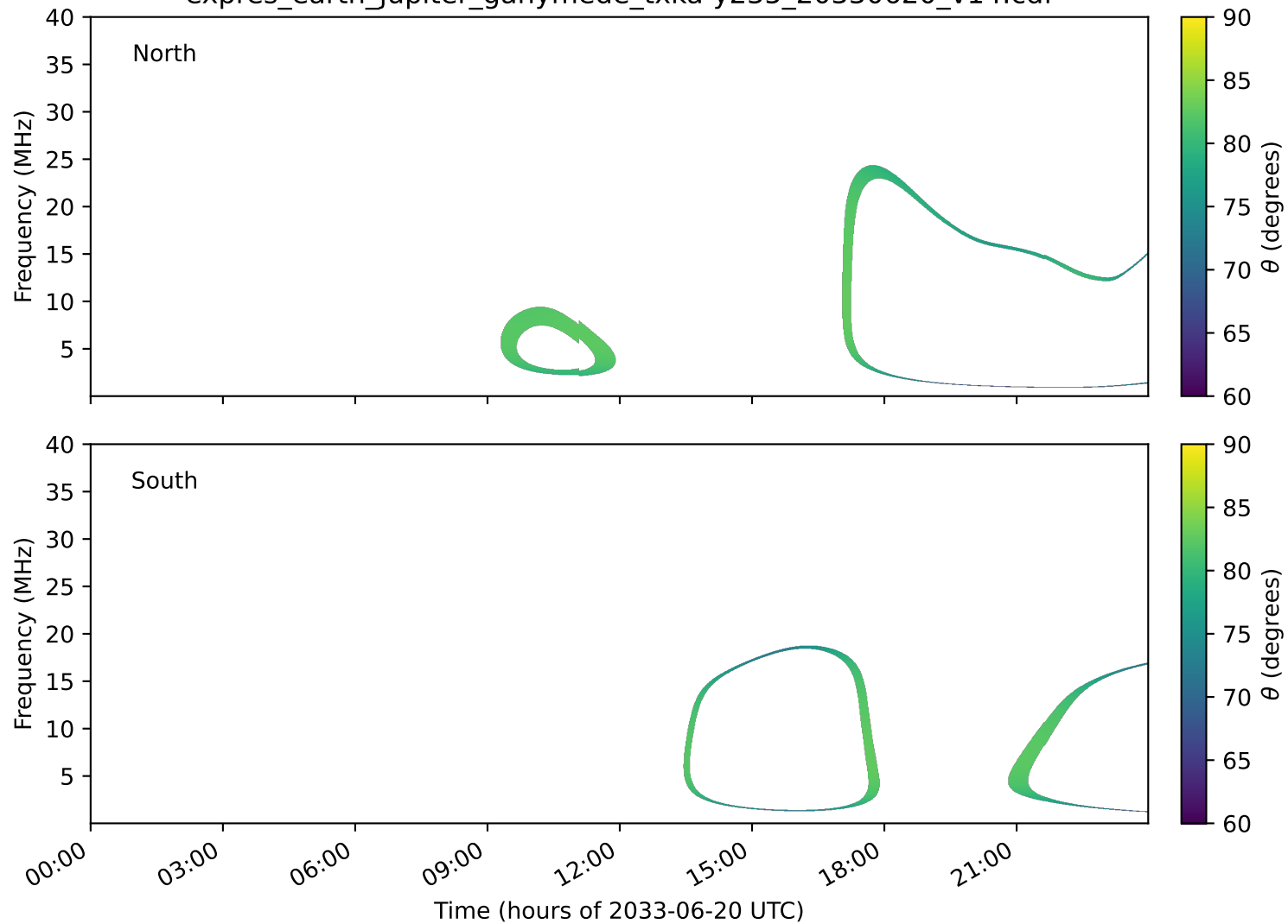
expres_earth_jupiter_ganymede_txka-y235_20330620_v14.cdf
