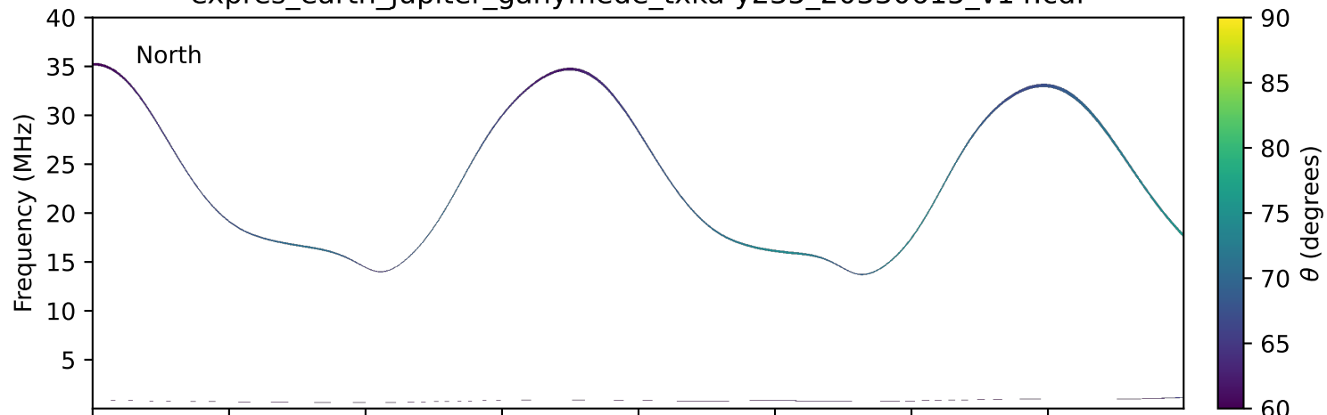
expres_earth_jupiter_ganymede_txka-y235_20330615_v14.cdf
