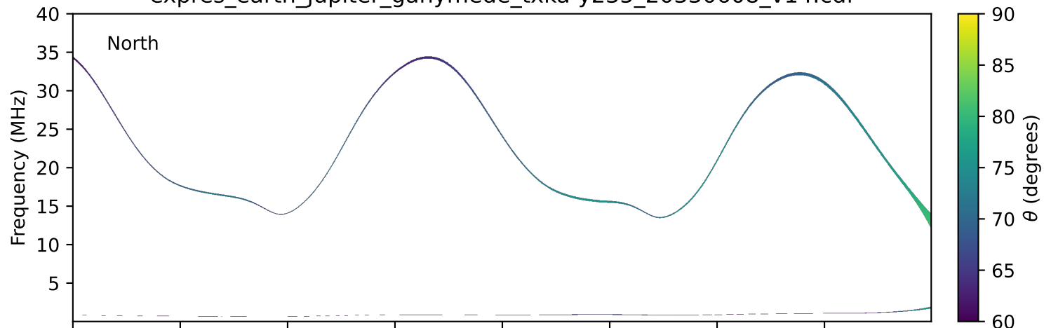
expres_earth_jupiter_ganymede_txka-y235_20330608_v14.cdf
