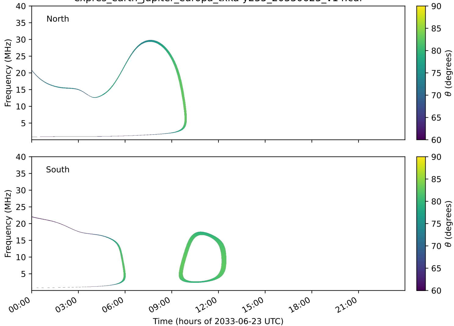
expres_earth_jupiter_europa_txka-y235_20330623_v14.cdf
