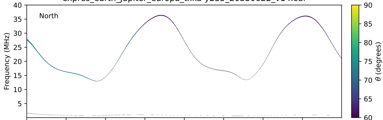
expres_earth_jupiter_europa_txka-y235_20330622_v14.cdf
