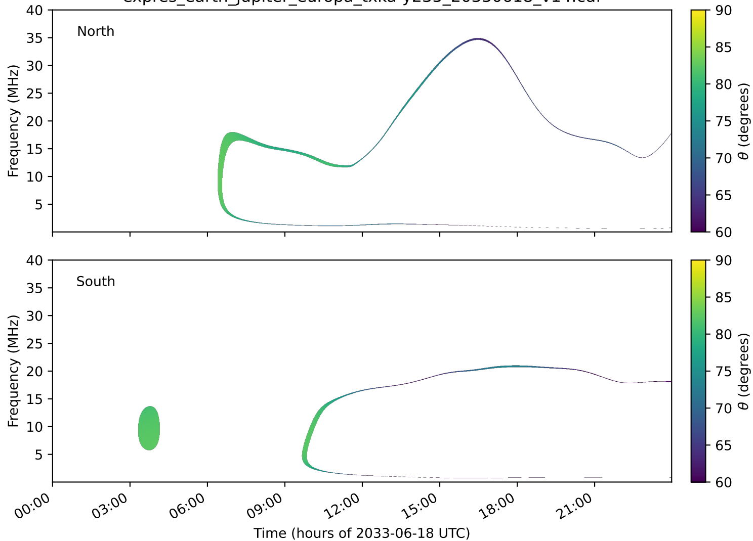
expres_earth_jupiter_europa_txka-y235_20330618_v14.cdf
