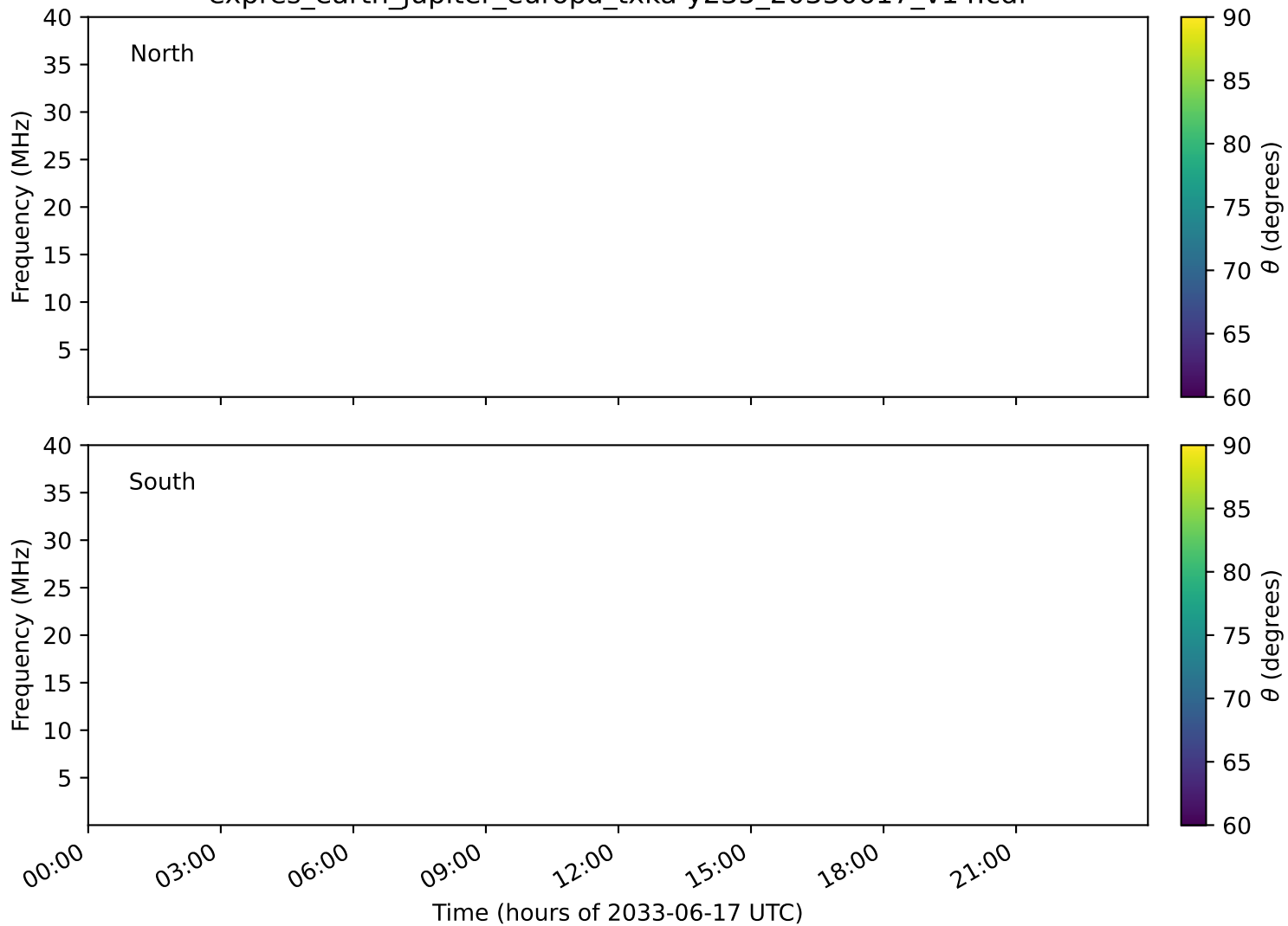
expres_earth_jupiter_europa_txka-y235_20330617_v14.cdf
