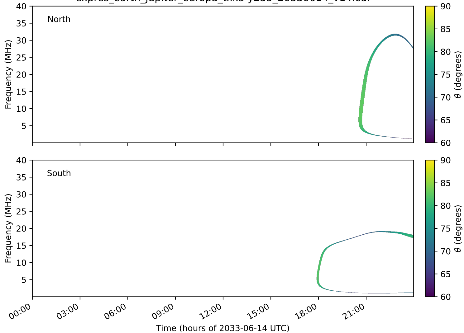
expres_earth_jupiter_europa_txka-y235_20330614_v14.cdf
