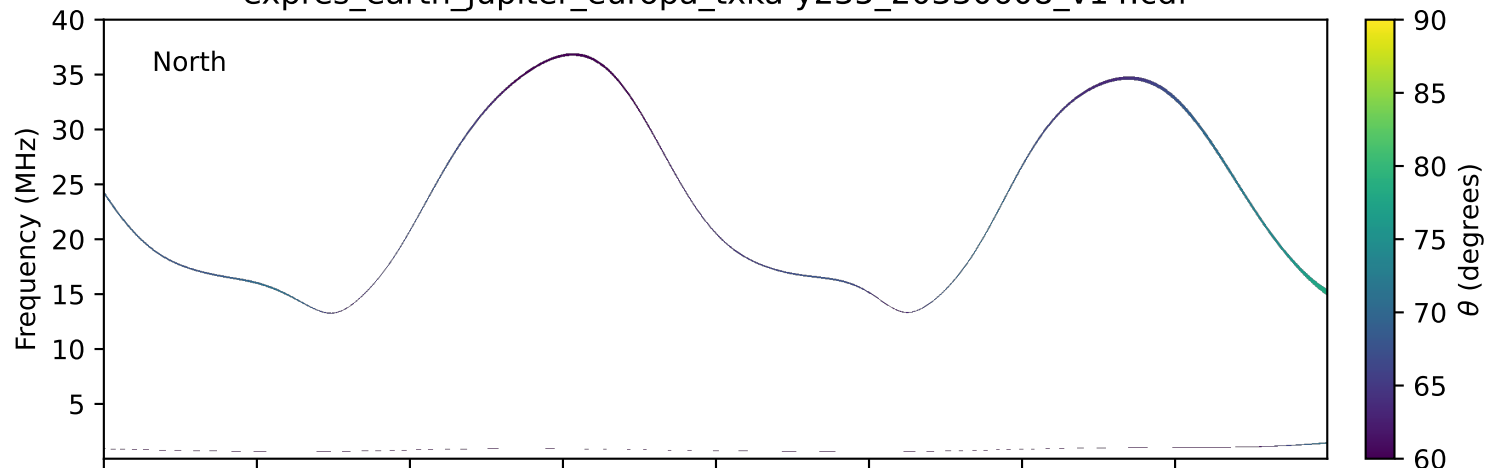
expres_earth_jupiter_europa_txka-y235_20330608_v14.cdf
