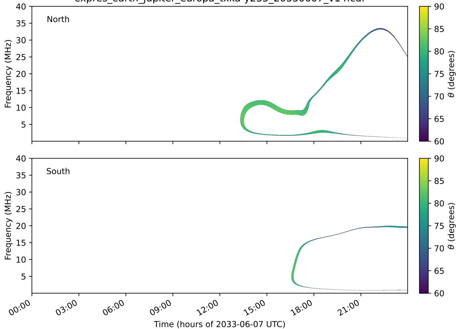
expres_earth_jupiter_europa_txka-y235_20330607_v14.cdf
