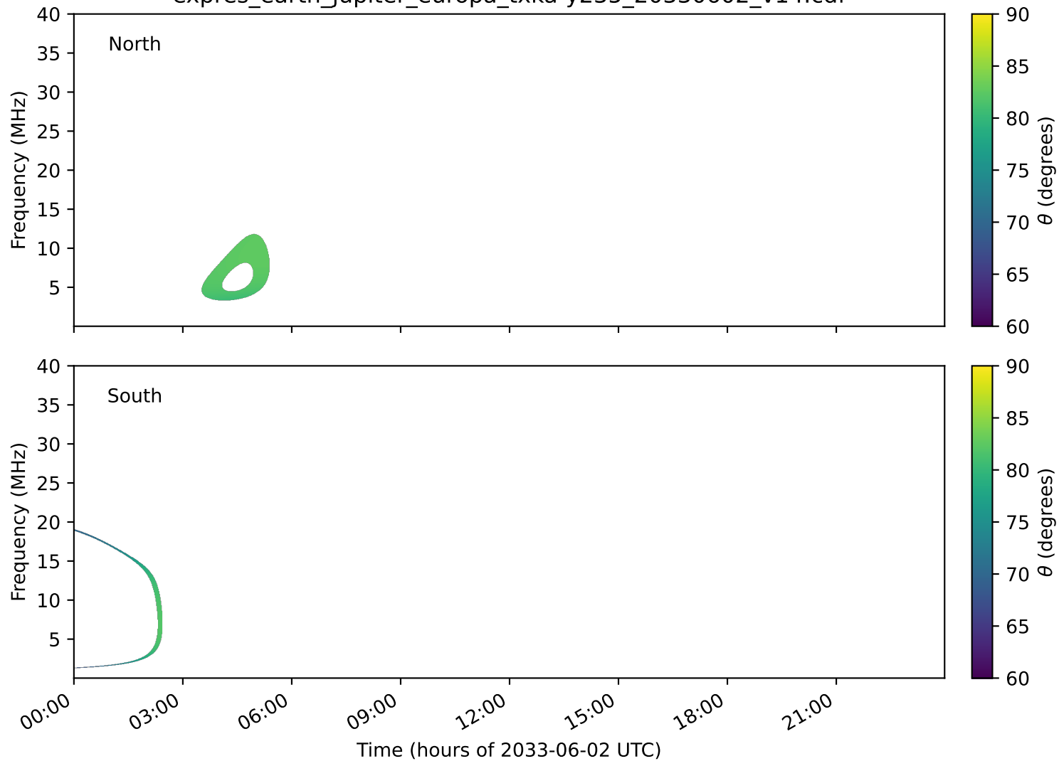
expres_earth_jupiter_europa_txka-y235_20330602_v14.cdf
