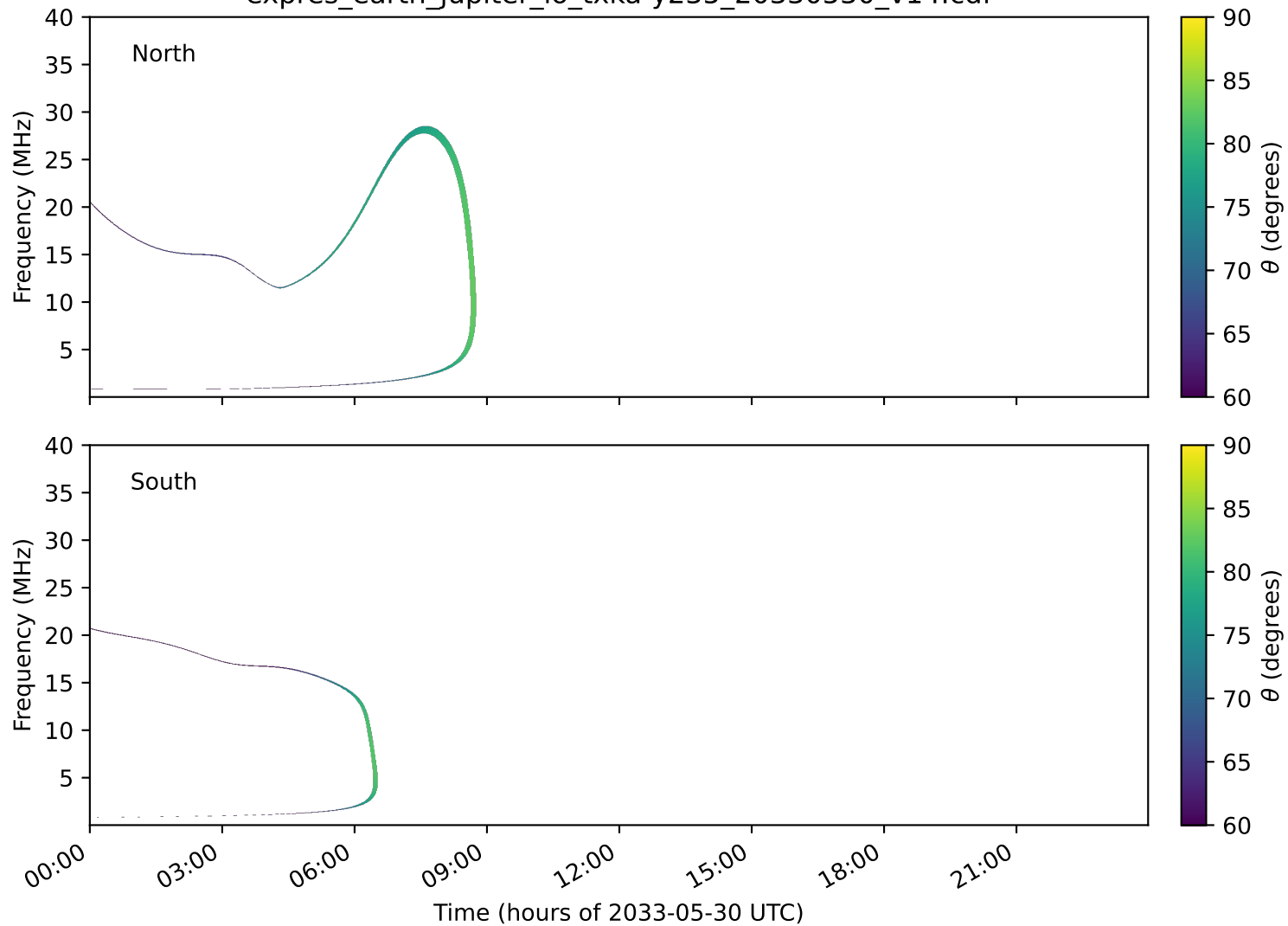
expres_earth_jupiter_io_txka-y235_20330530_v14.cdf
