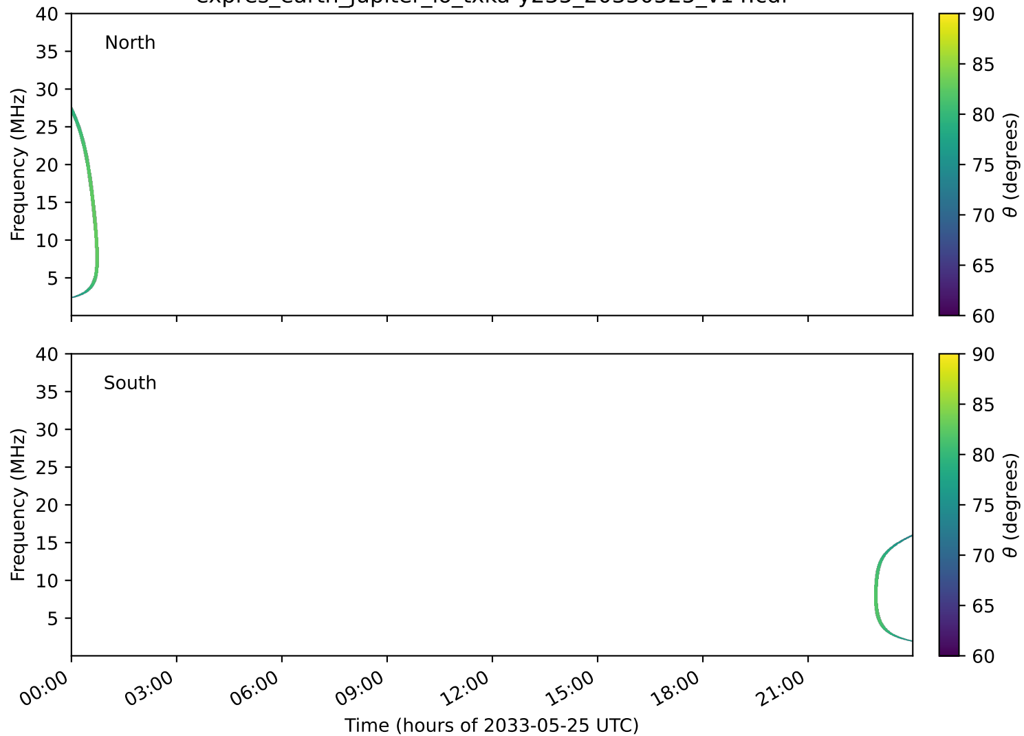
expres_earth_jupiter_io_txka-y235_20330525_v14.cdf
