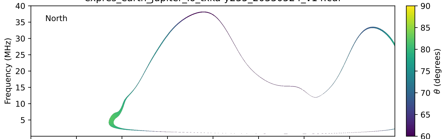
expres_earth_jupiter_io_txka-y235_20330524_v14.cdf
