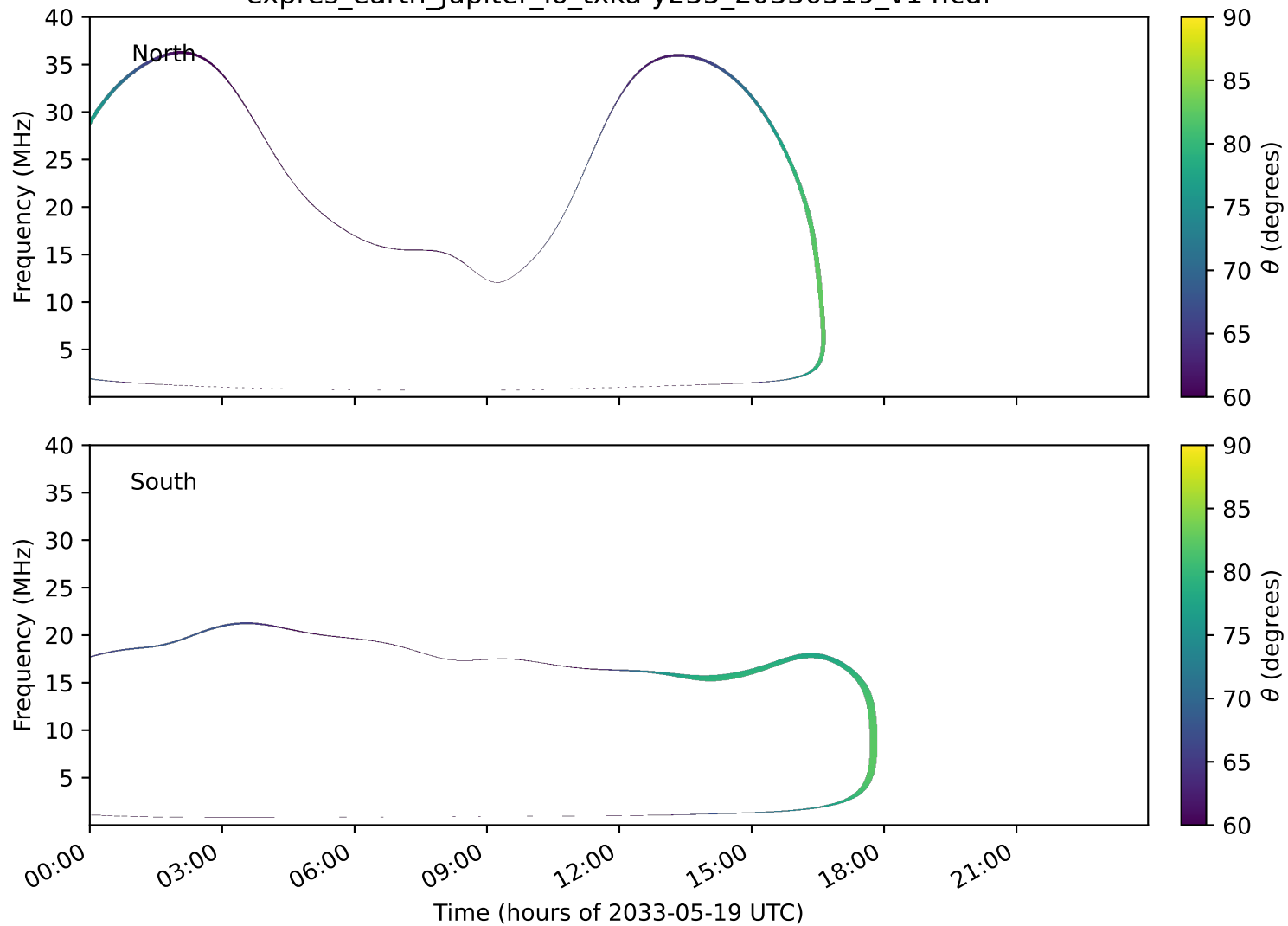
expres_earth_jupiter_io_txka-y235_20330519_v14.cdf
