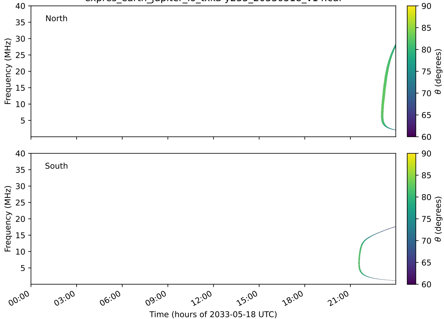
expres_earth_jupiter_io_txka-y235_20330518_v14.cdf
