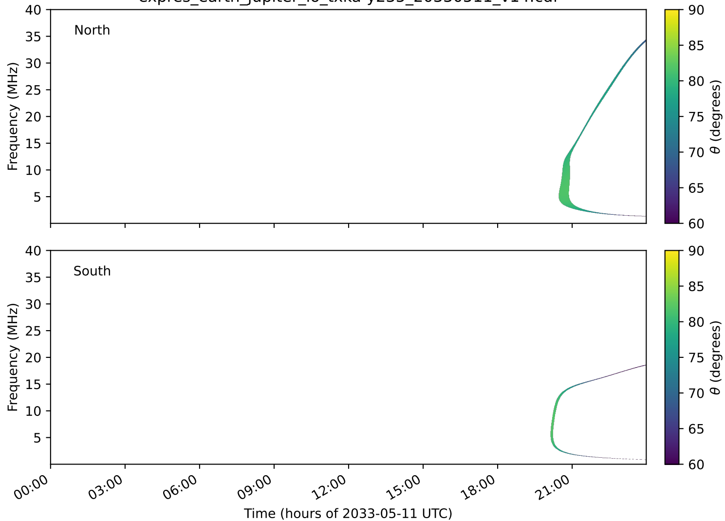
expres_earth_jupiter_io_txka-y235_20330511_v14.cdf
