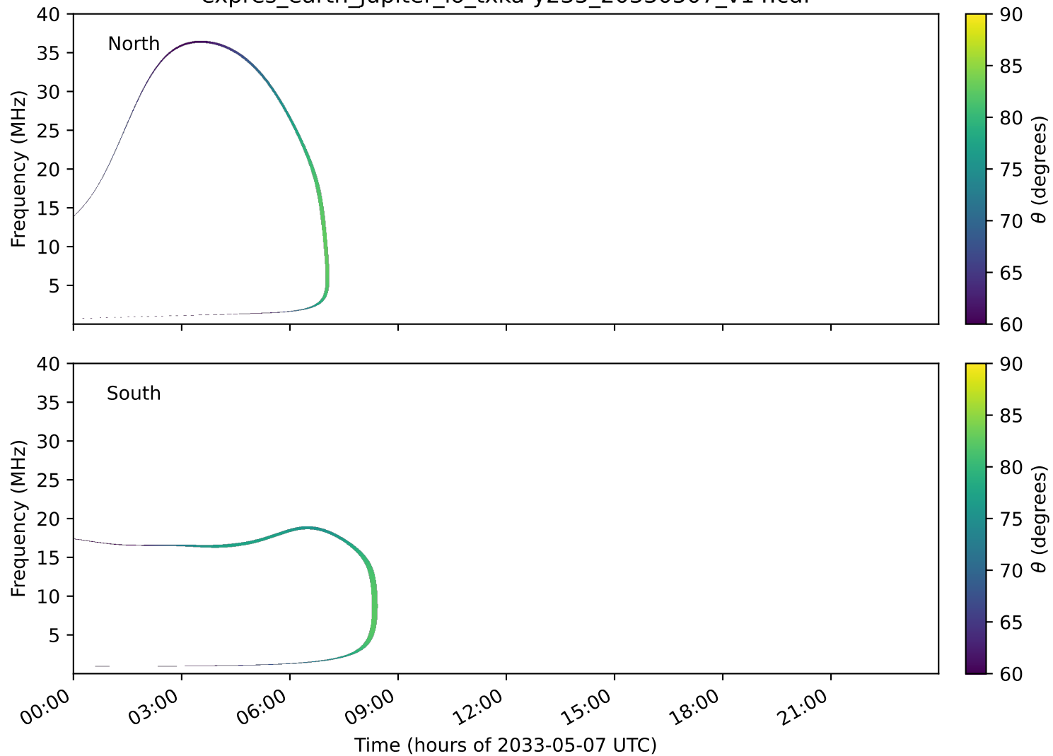
expres_earth_jupiter_io_txka-y235_20330507_v14.cdf
