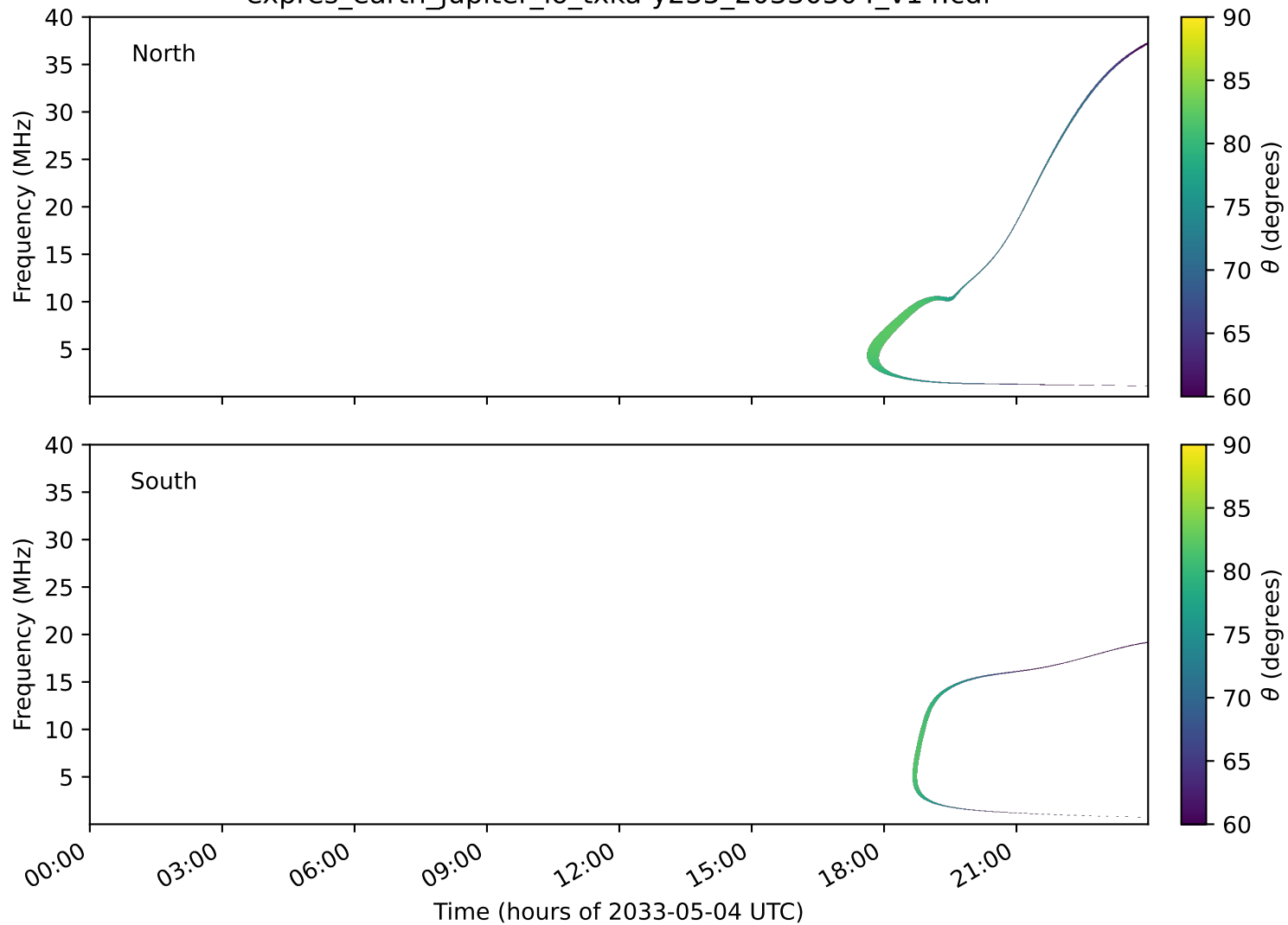
expres_earth_jupiter_io_txka-y235_20330504_v14.cdf
