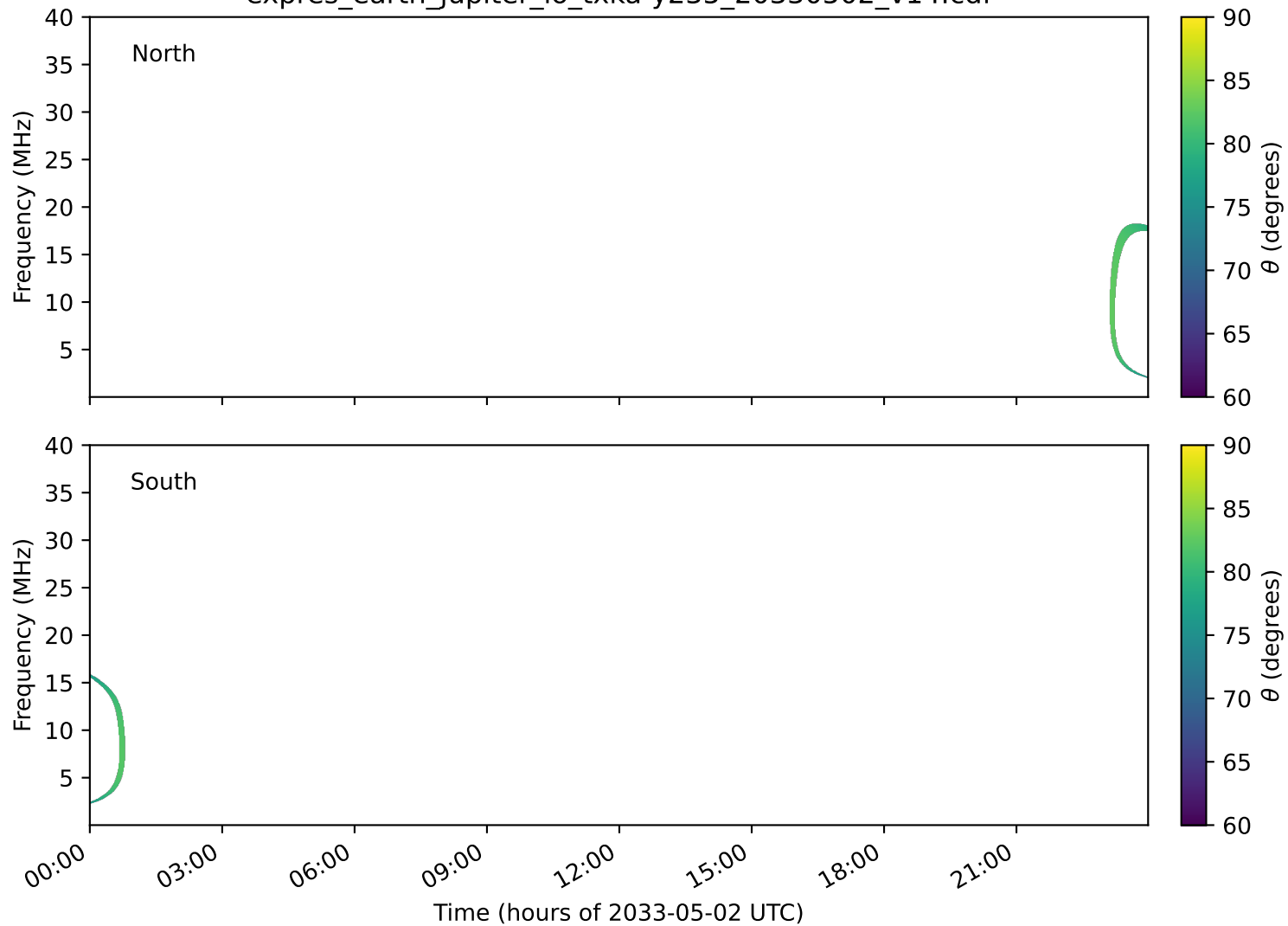
expres_earth_jupiter_io_txka-y235_20330502_v14.cdf
