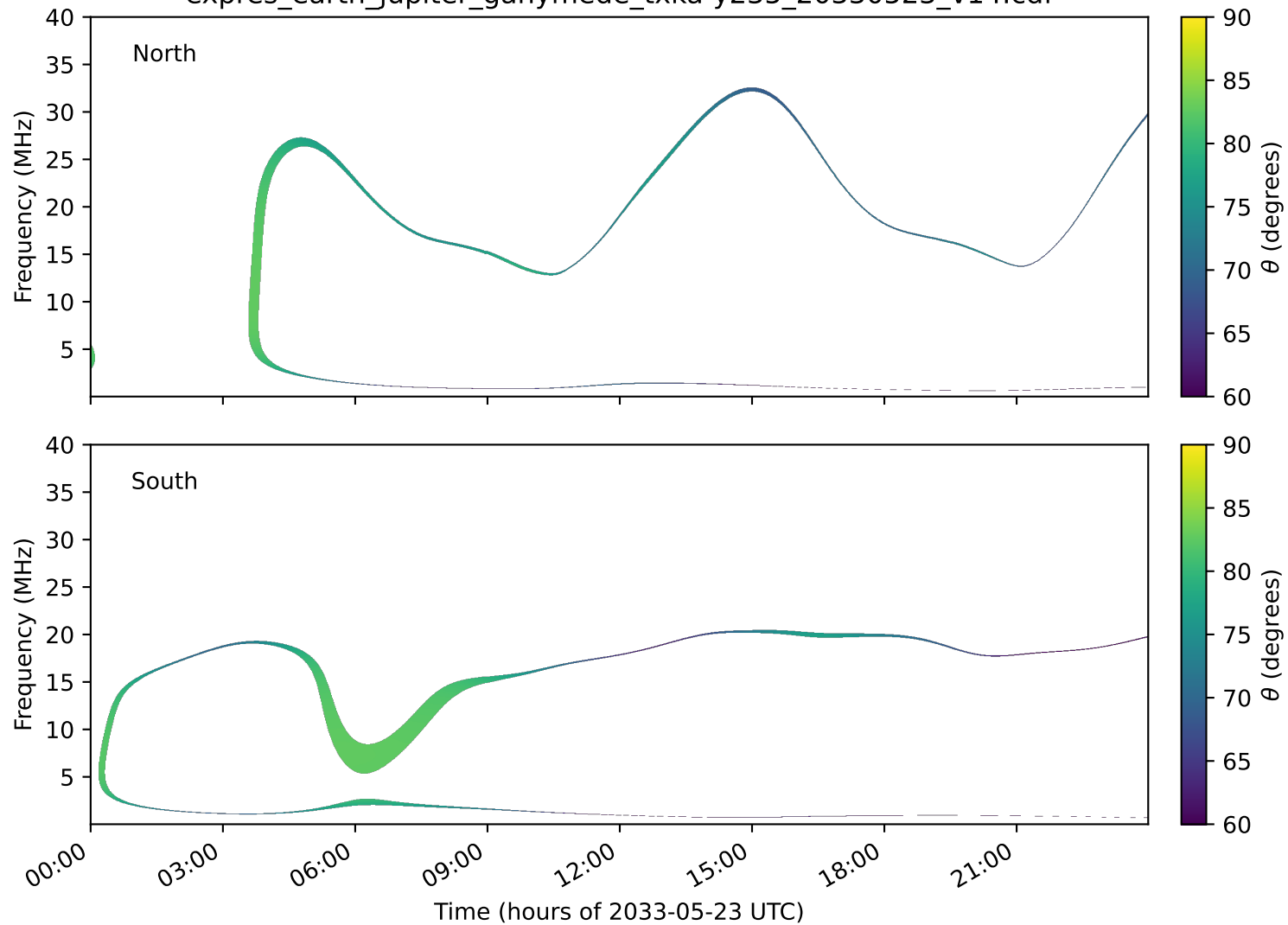
expres_earth_jupiter_ganymede_txka-y235_20330523_v14.cdf
