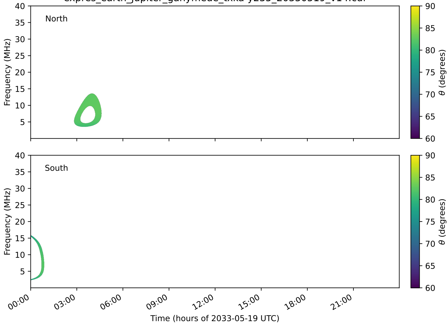
expres_earth_jupiter_ganymede_txka-y235_20330519_v14.cdf
