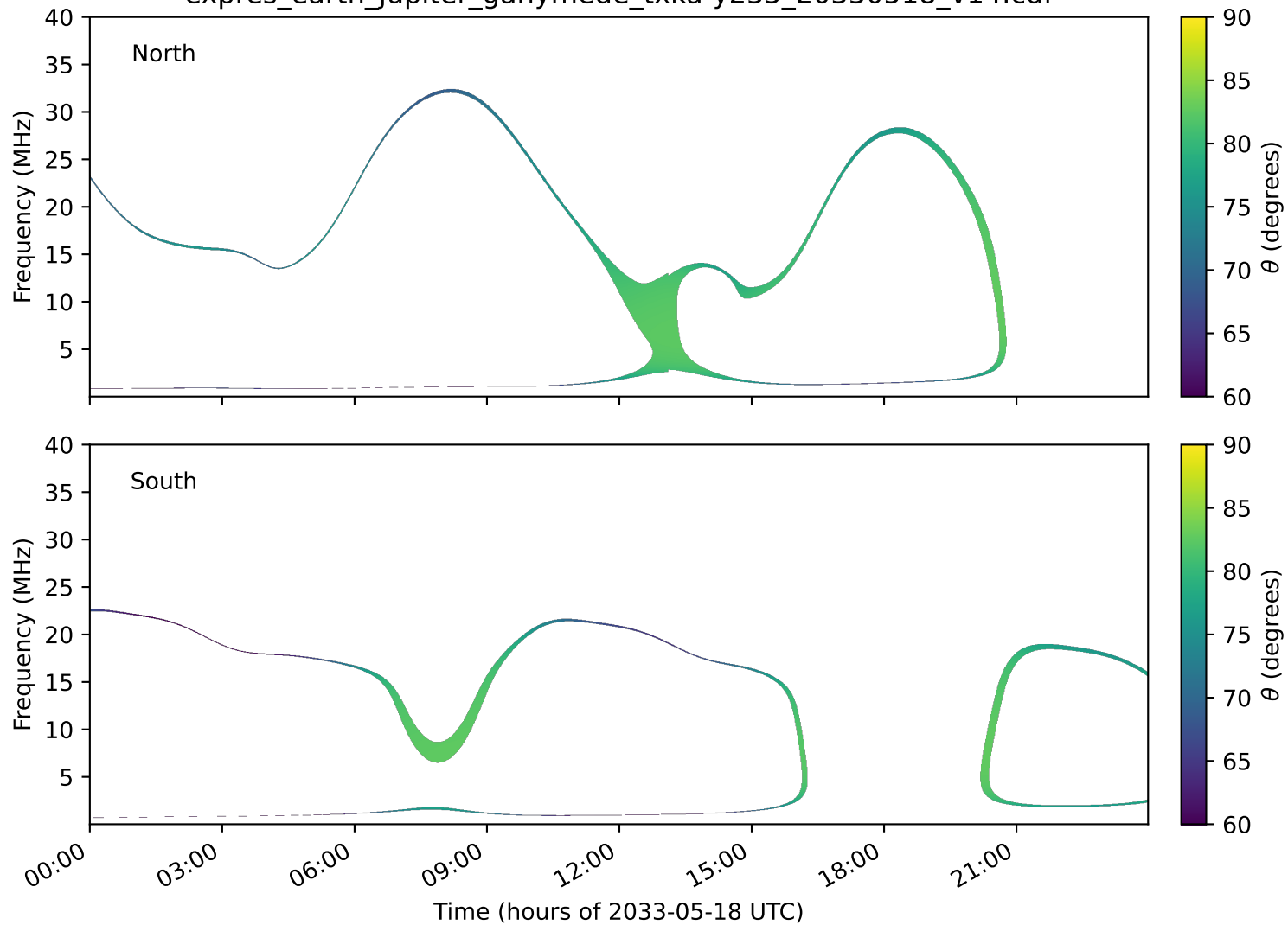
expres_earth_jupiter_ganymede_txka-y235_20330518_v14.cdf
