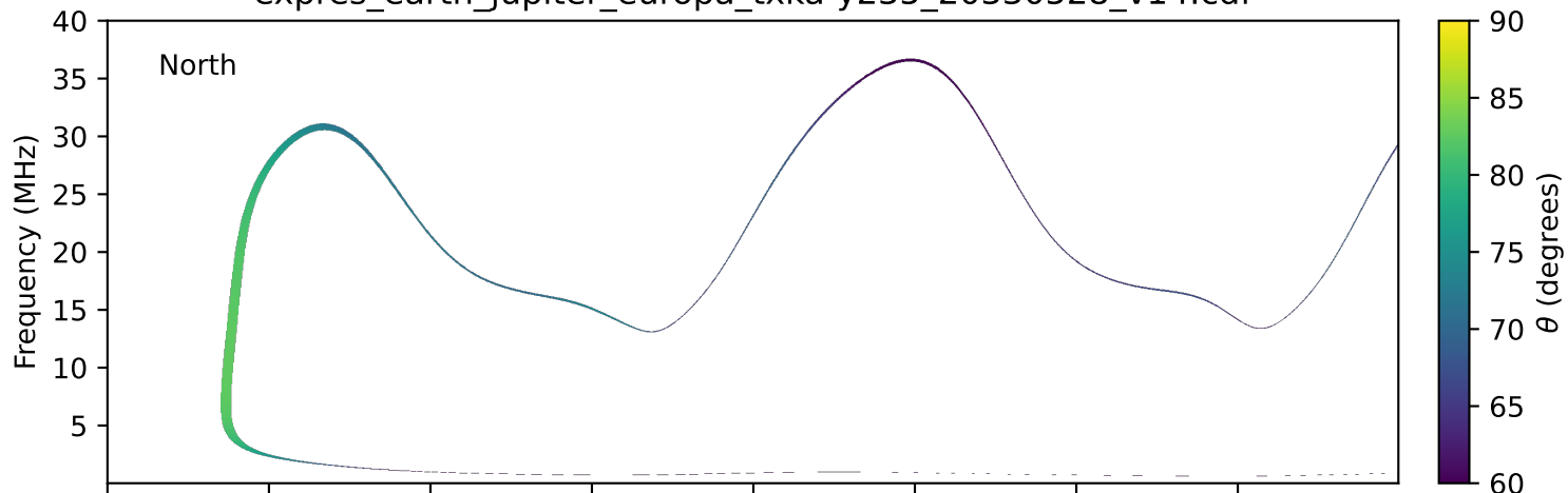
expres_earth_jupiter_europa_txka-y235_20330528_v14.cdf
