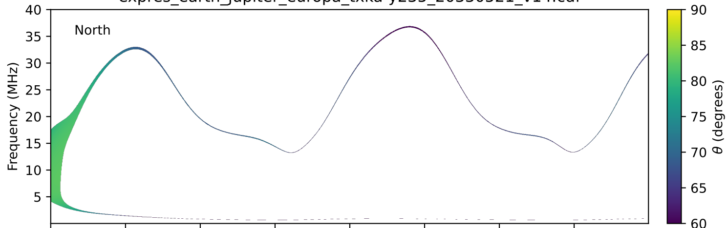
expres_earth_jupiter_europa_txka-y235_20330521_v14.cdf
