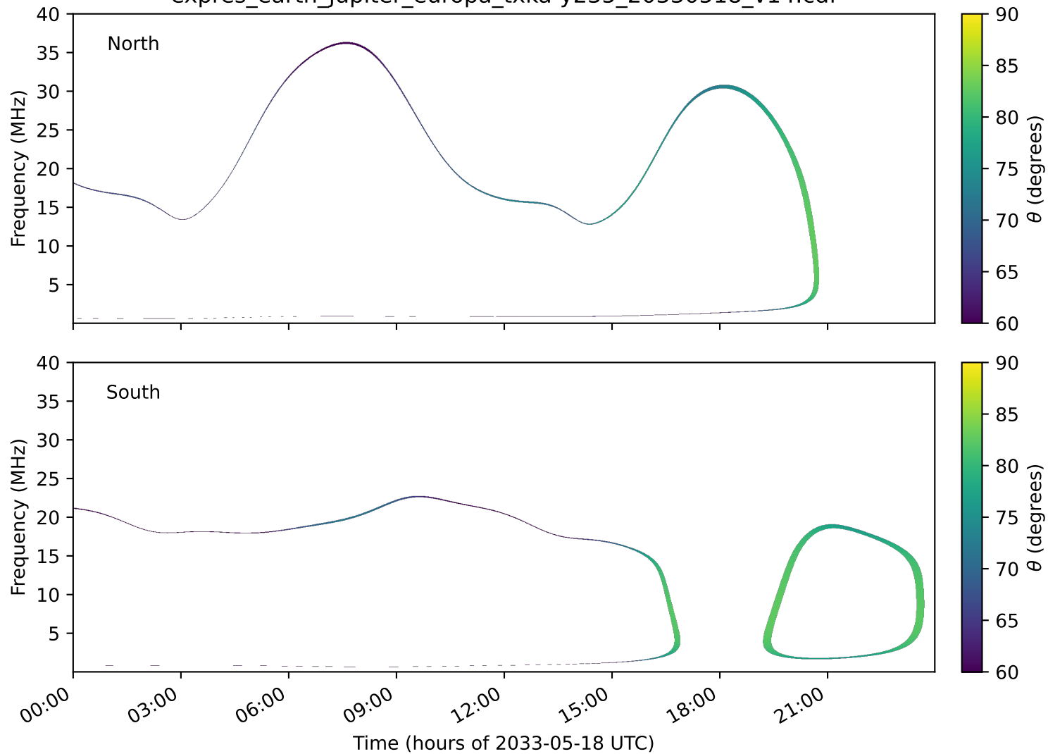
expres_earth_jupiter_europa_txka-y235_20330518_v14.cdf
