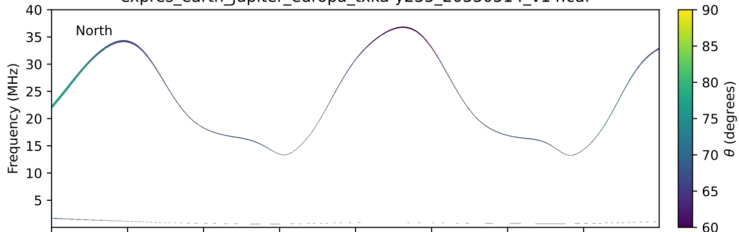
expres_earth_jupiter_europa_txka-y235_20330514_v14.cdf
