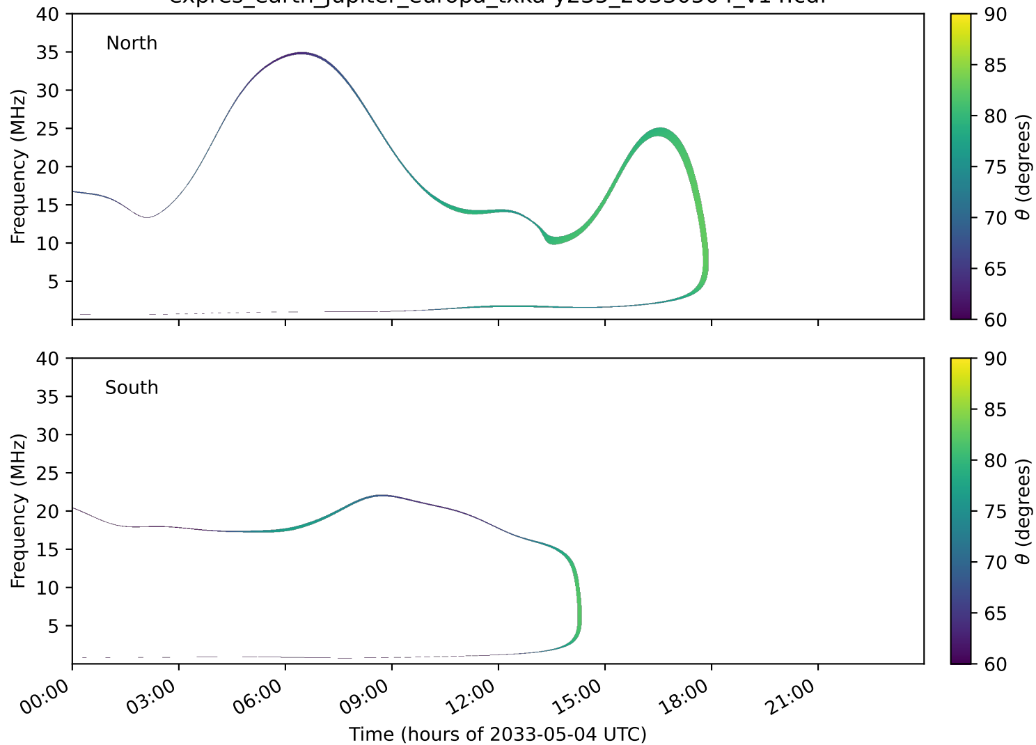
expres_earth_jupiter_europa_txka-y235_20330504_v14.cdf
