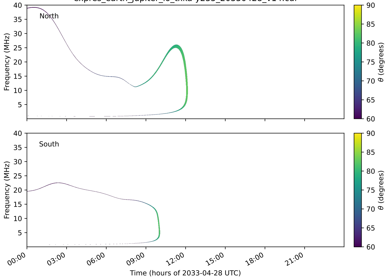
expres_earth_jupiter_io_txka-y235_20330428_v14.cdf
