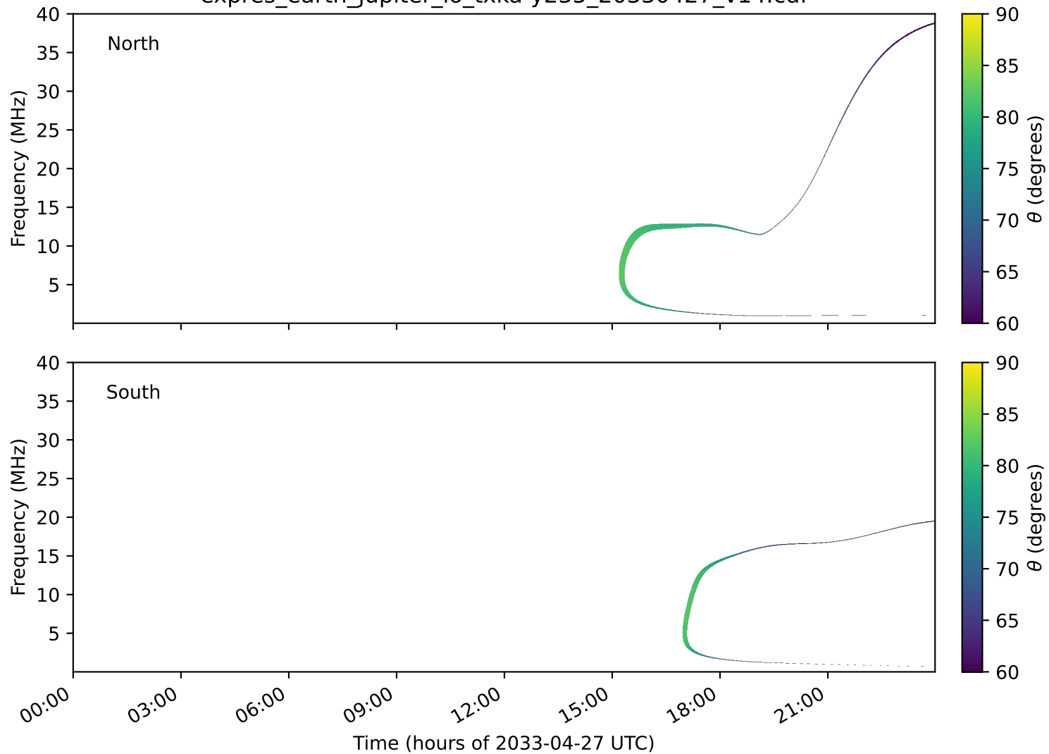
expres_earth_jupiter_io_txka-y235_20330427_v14.cdf
