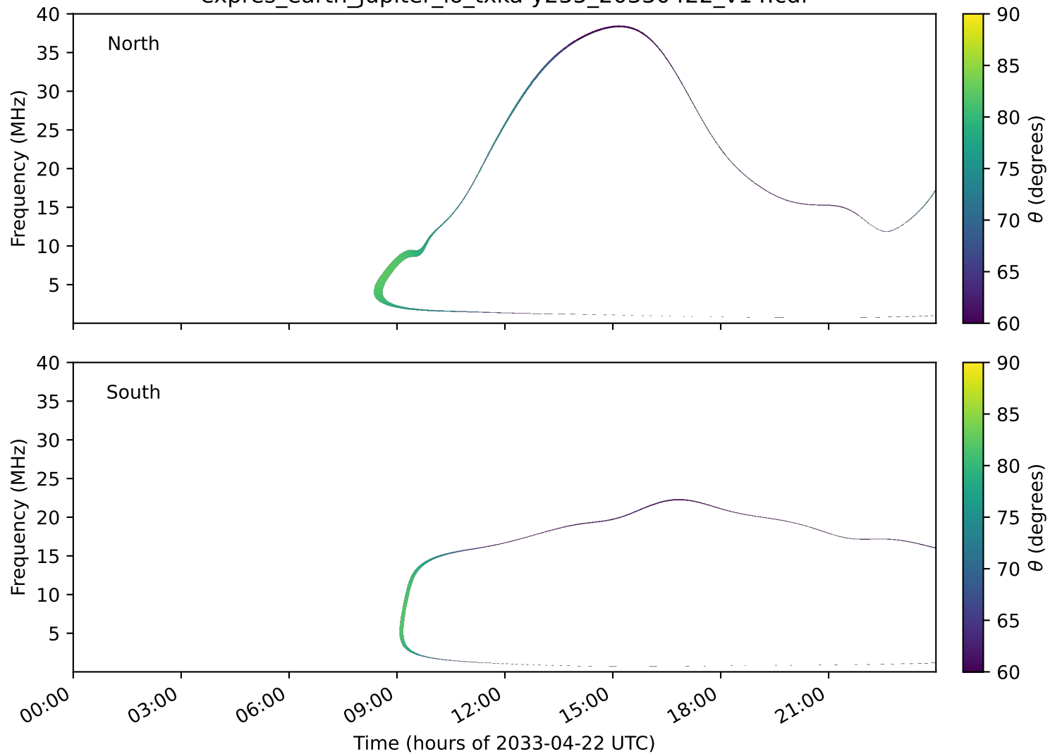
expres_earth_jupiter_io_txka-y235_20330422_v14.cdf
