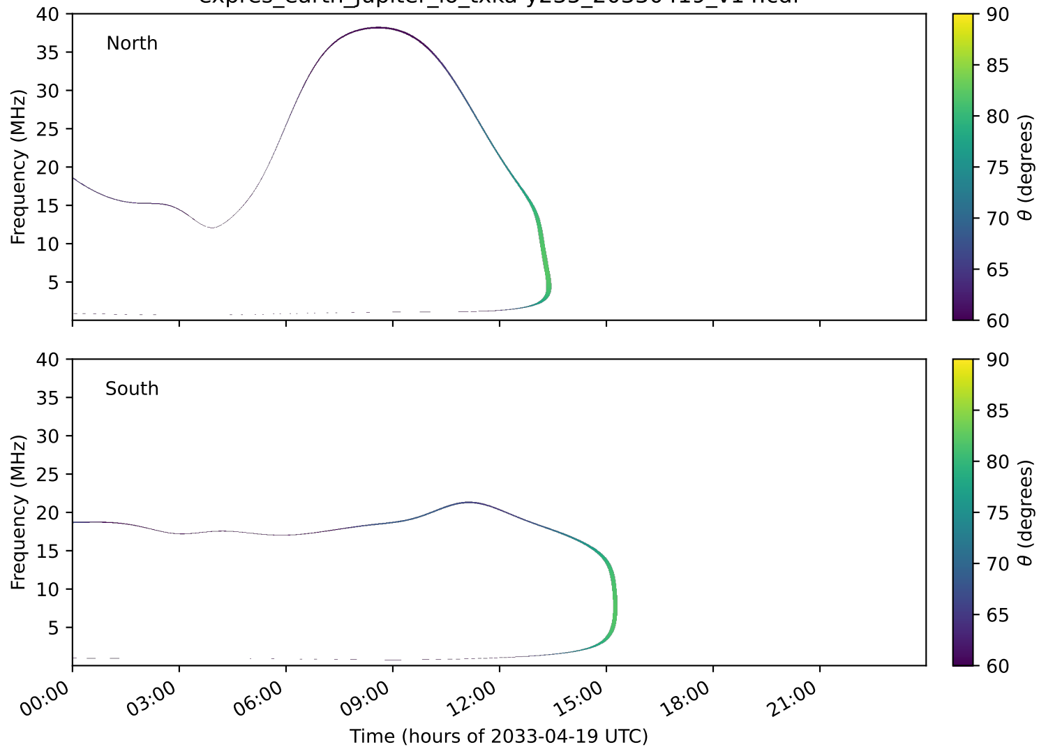
expres_earth_jupiter_io_txka-y235_20330419_v14.cdf
