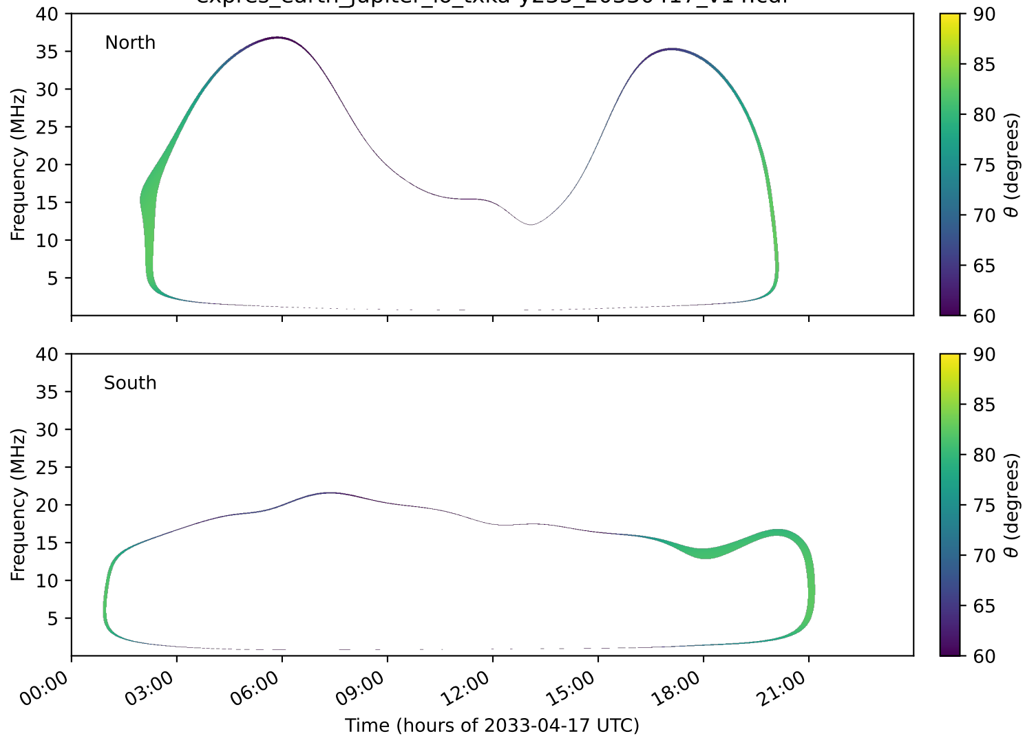
expres_earth_jupiter_io_txka-y235_20330417_v14.cdf
