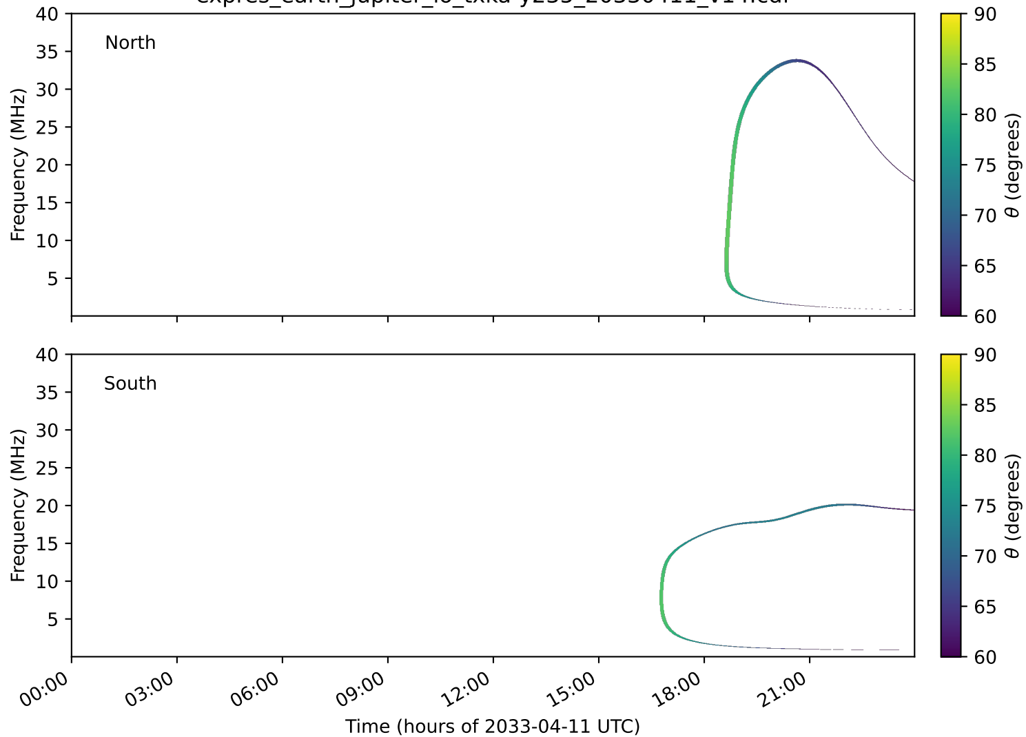
expres_earth_jupiter_io_txka-y235_20330411_v14.cdf
