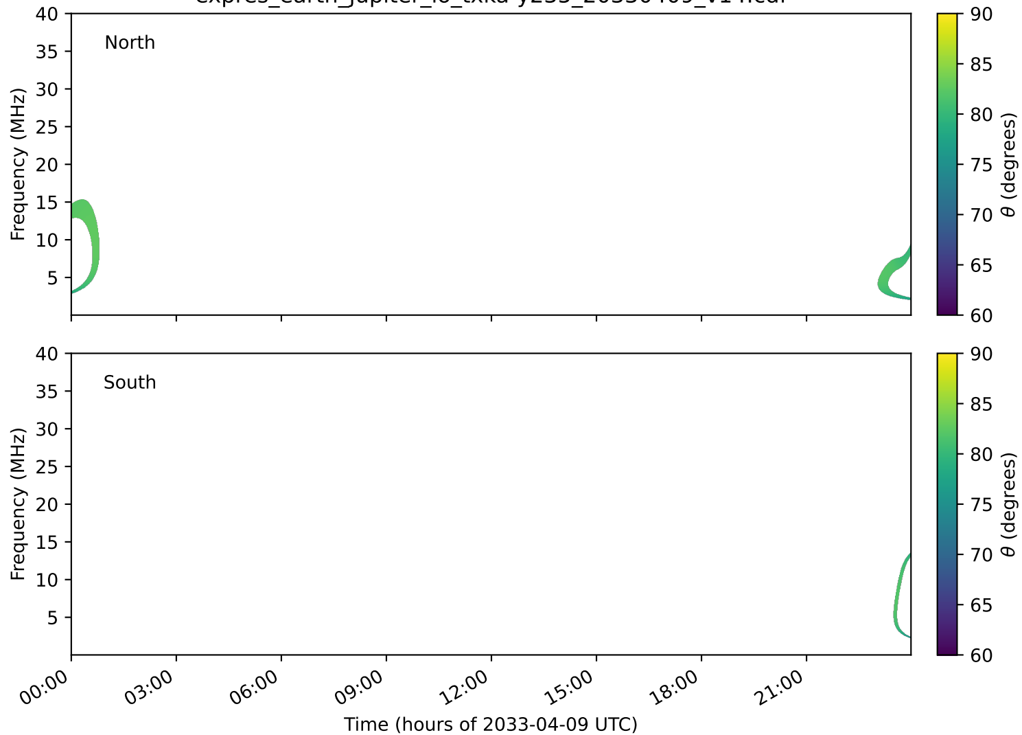
expres_earth_jupiter_io_txka-y235_20330409_v14.cdf
