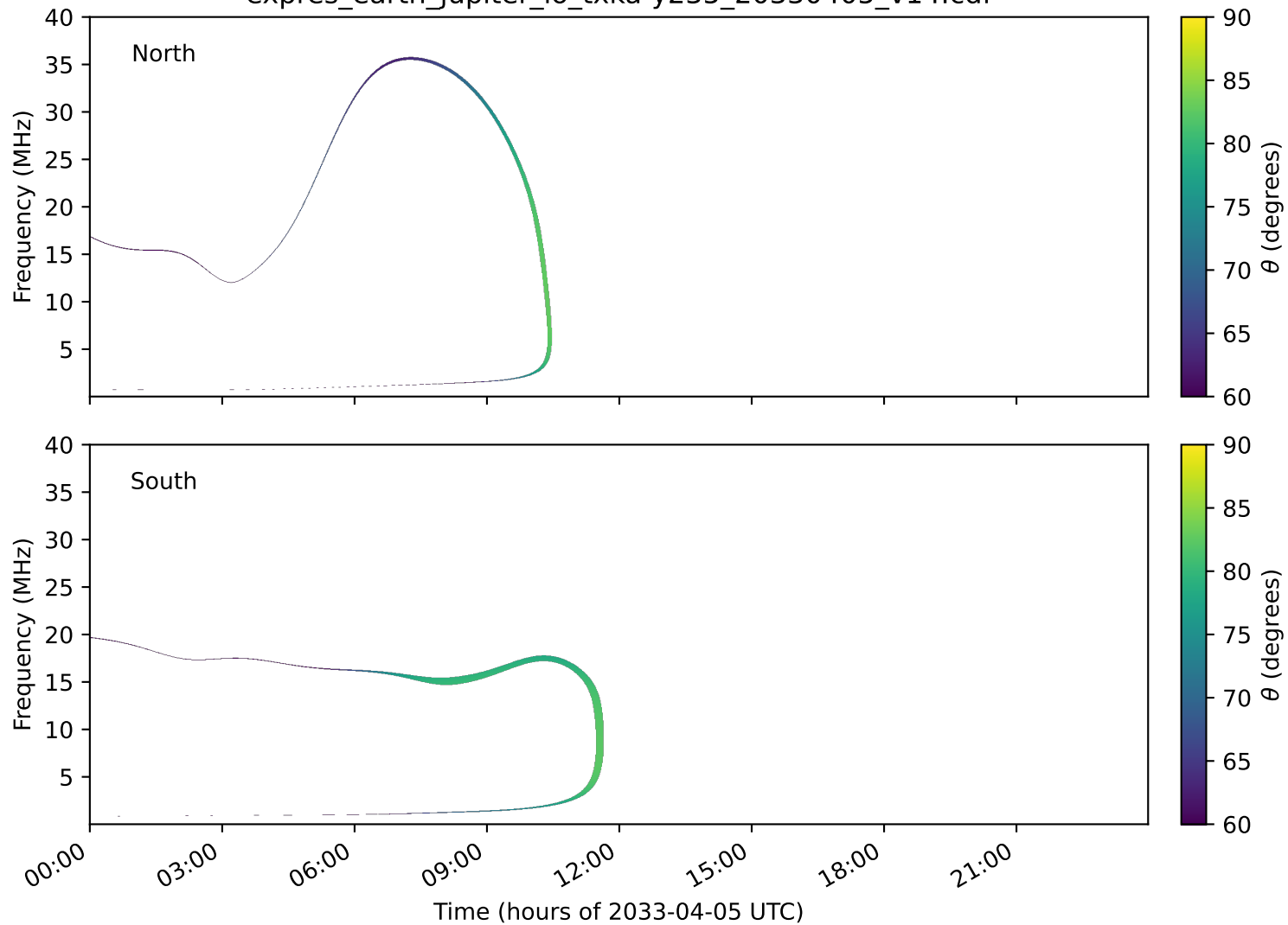
expres_earth_jupiter_io_txka-y235_20330405_v14.cdf
