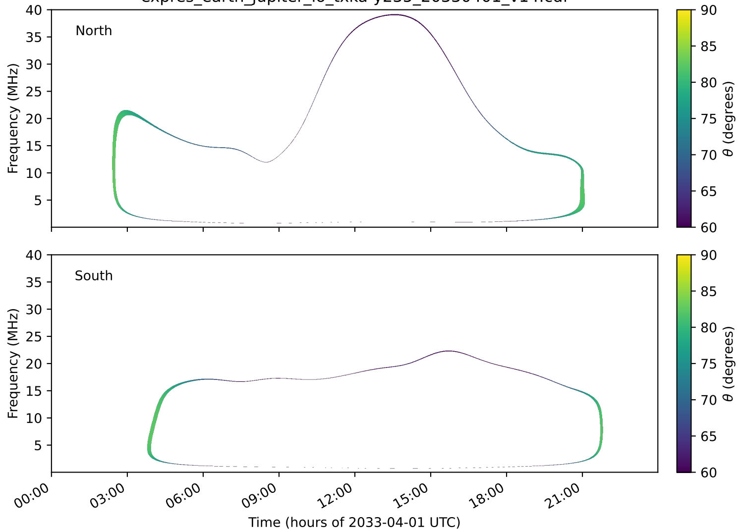
expres_earth_jupiter_io_txka-y235_20330401_v14.cdf
