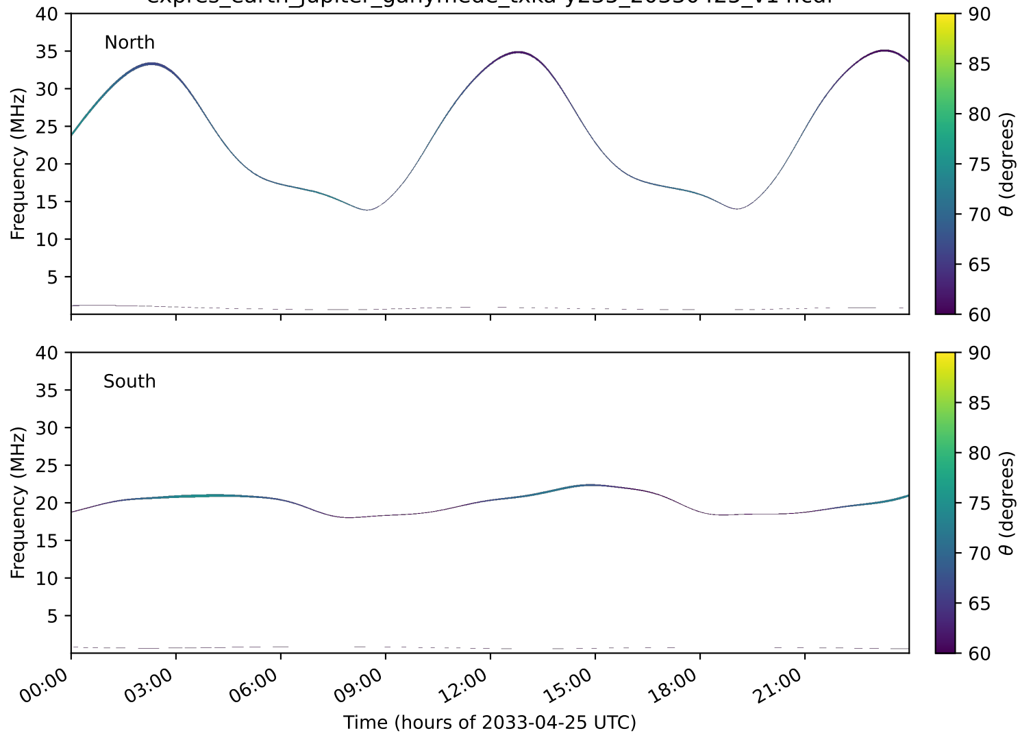
expres_earth_jupiter_ganymede_txka-y235_20330425_v14.cdf
