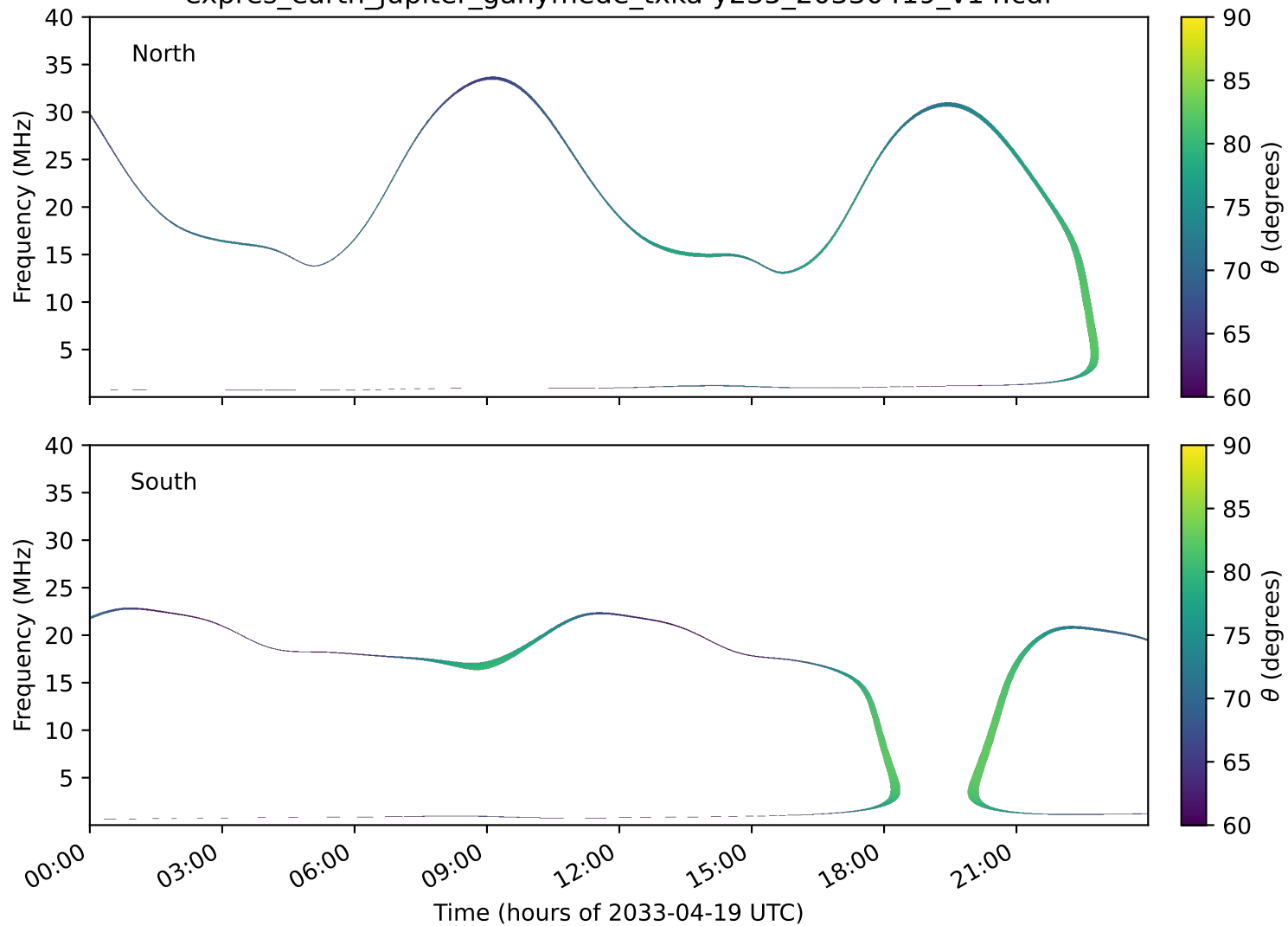
expres_earth_jupiter_ganymede_txka-y235_20330419_v14.cdf
