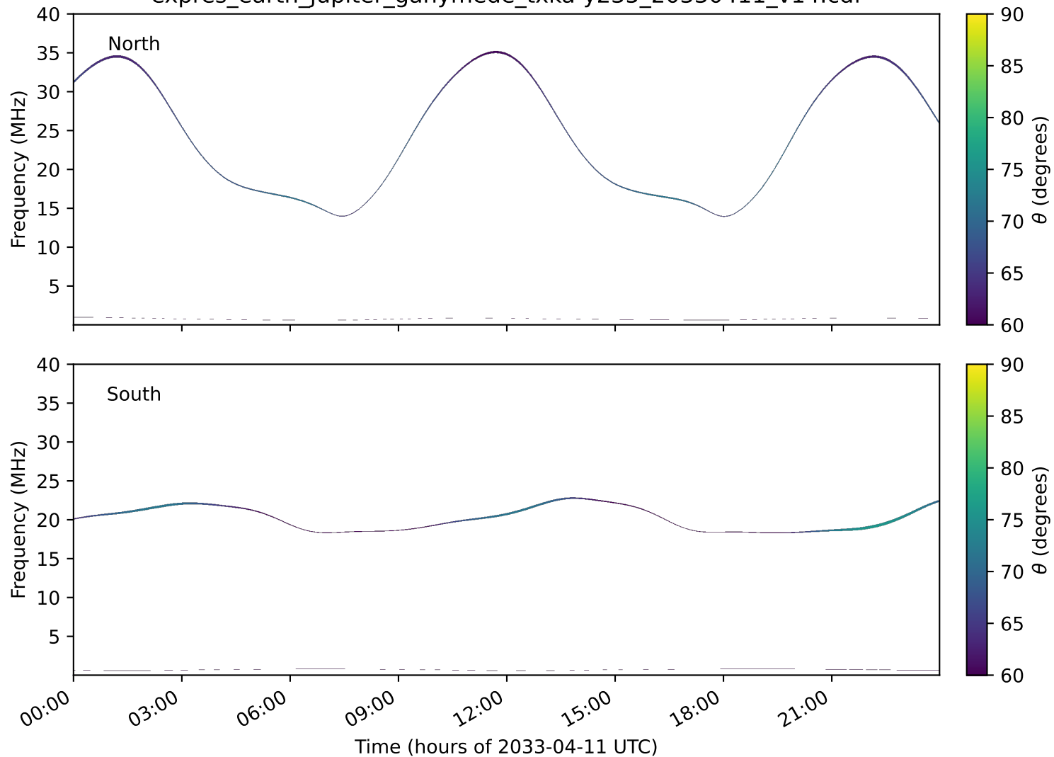
expres_earth_jupiter_ganymede_txka-y235_20330411_v14.cdf
