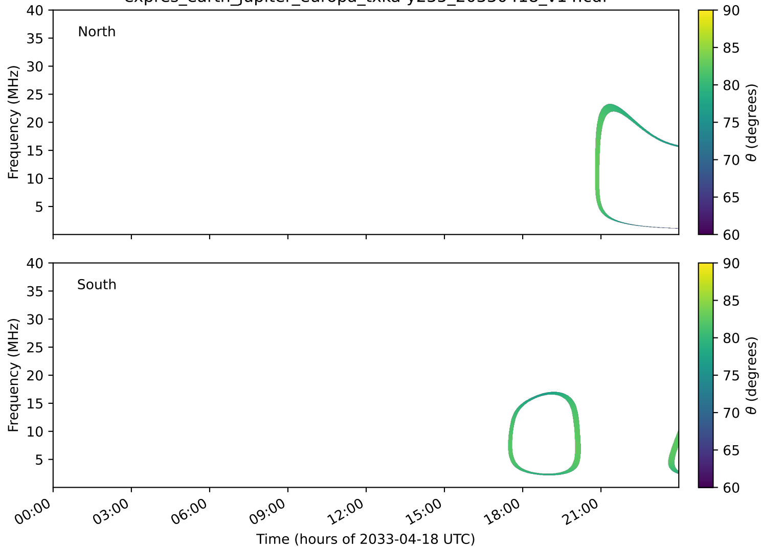
expres_earth_jupiter_europa_txka-y235_20330418_v14.cdf
