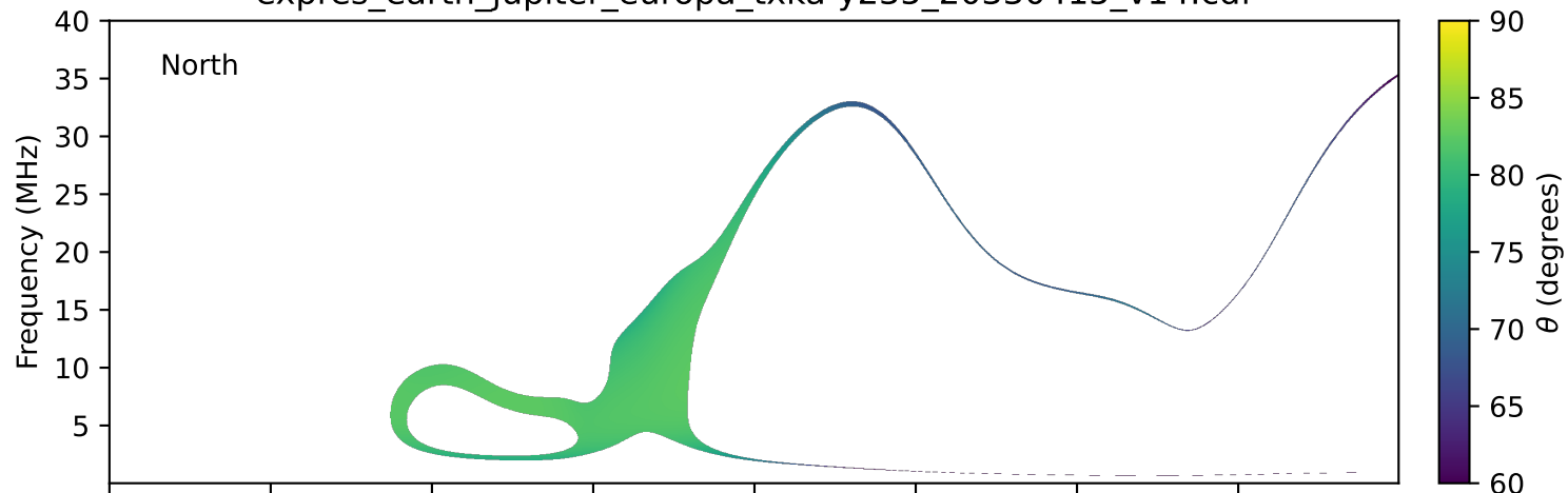
expres_earth_jupiter_europa_txka-y235_20330415_v14.cdf
