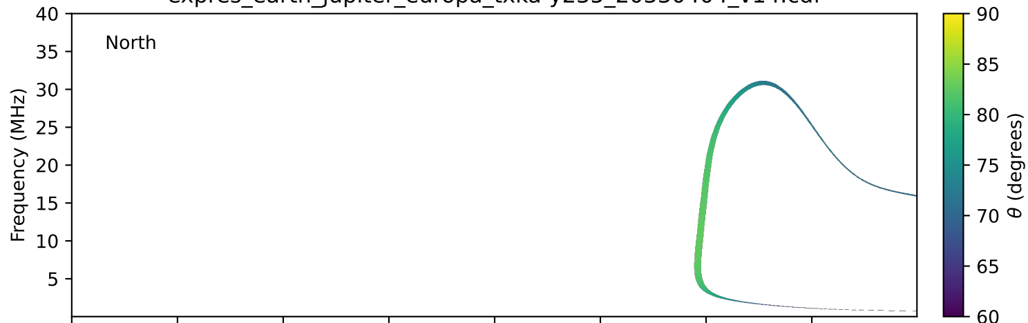
expres_earth_jupiter_europa_txka-y235_20330404_v14.cdf
