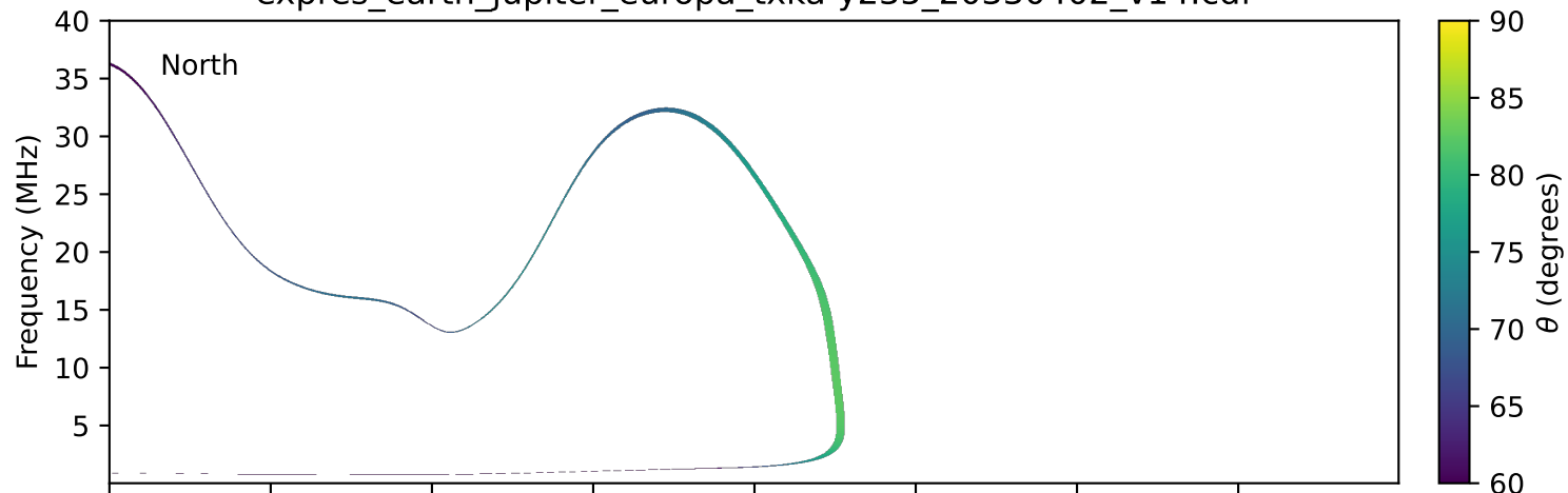
expres_earth_jupiter_europa_txka-y235_20330402_v14.cdf
