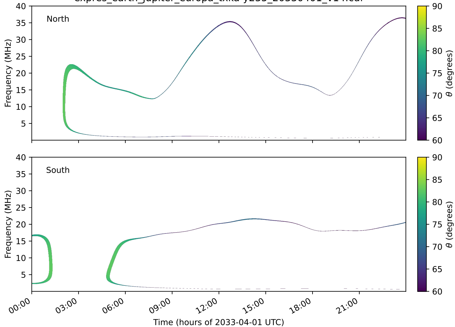
expres_earth_jupiter_europa_txka-y235_20330401_v14.cdf
