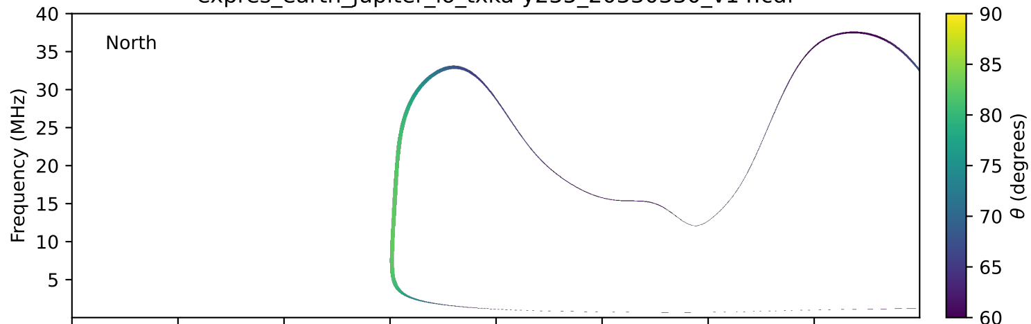
expres_earth_jupiter_io_txka-y235_20330330_v14.cdf
