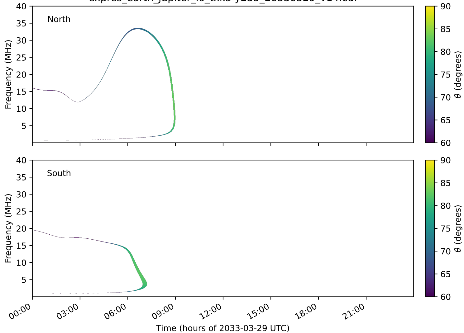
expres_earth_jupiter_io_txka-y235_20330329_v14.cdf
