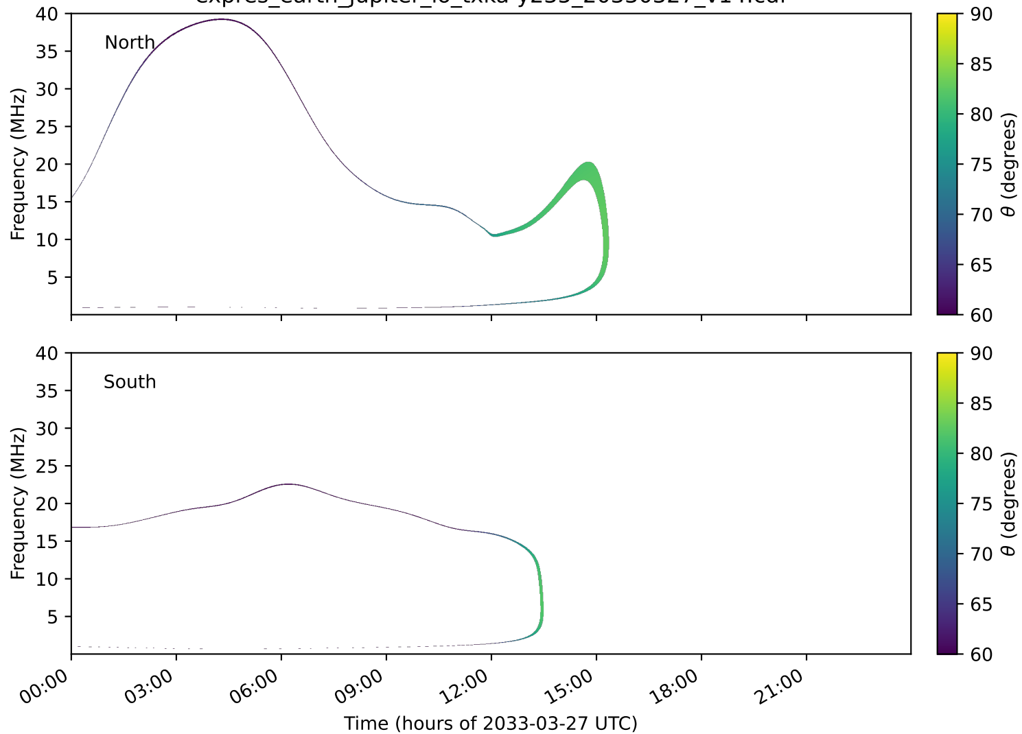
expres_earth_jupiter_io_txka-y235_20330327_v14.cdf
