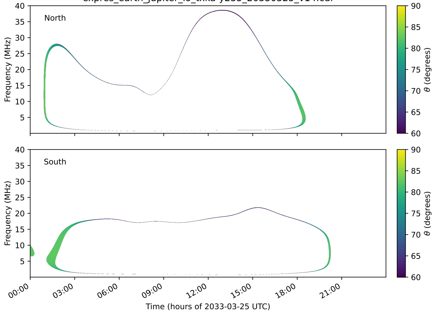
expres_earth_jupiter_io_txka-y235_20330325_v14.cdf
